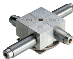
FL6xx-xxxx-xx04 Adjustable tool for enamelling flat wire
