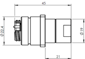
euMicron Receptacle Flange Mount
